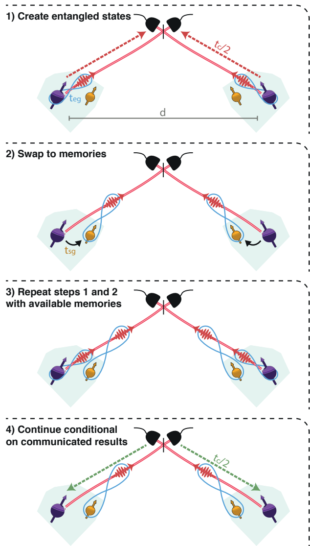
FIG. 2. Multiplexing concept. The protocol starts with a creation of local entanglement between the broker qubits and single photons at both nodes (step 1). The state of the broker qubits is then immediately transferred to the memory qubits (step 2), which allows for a second entanglement attempt before the result of the first one is known (step 3). Once the signal heralding success or failure of the attempt is received at the nodes, the occupied memories can be reused for new attempts (step 4).
